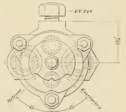
PLAN VIEW OF DUPLEX BRAKE VALVE.
